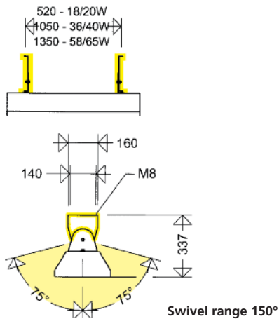
Swivel range 150°
